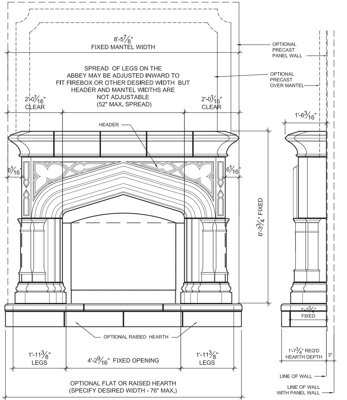
A ELEVATION - ABBEY FIREPLACE 1/2" = 1'-0"
