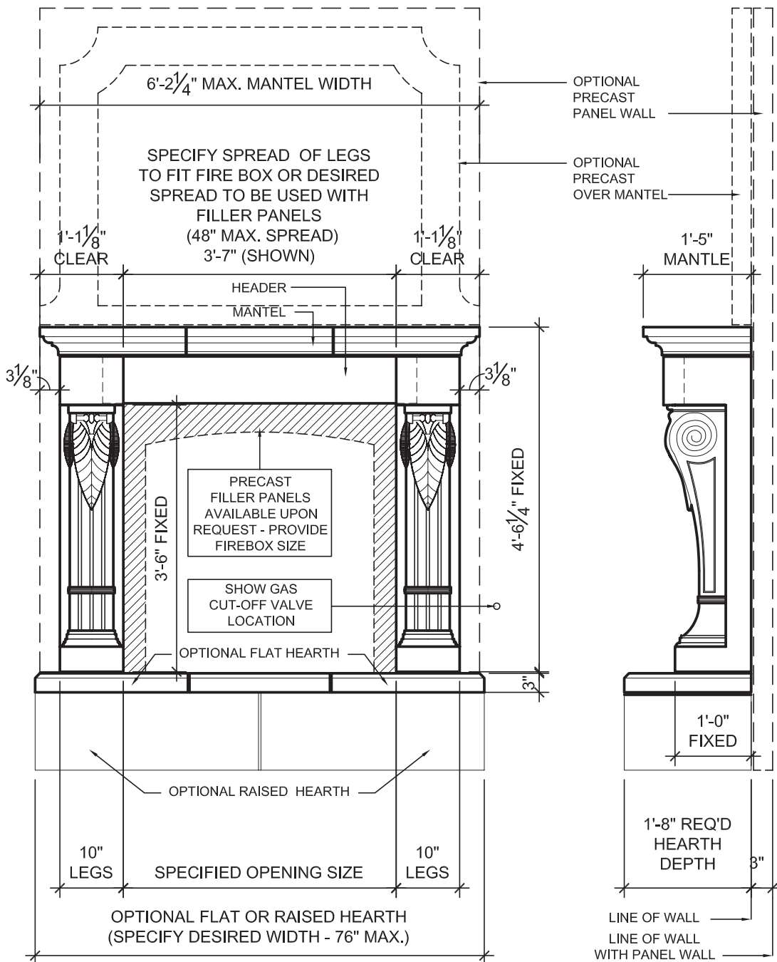
A ELEVATION - ATHENS FIREPLACE 1/2" = 1'-0"
