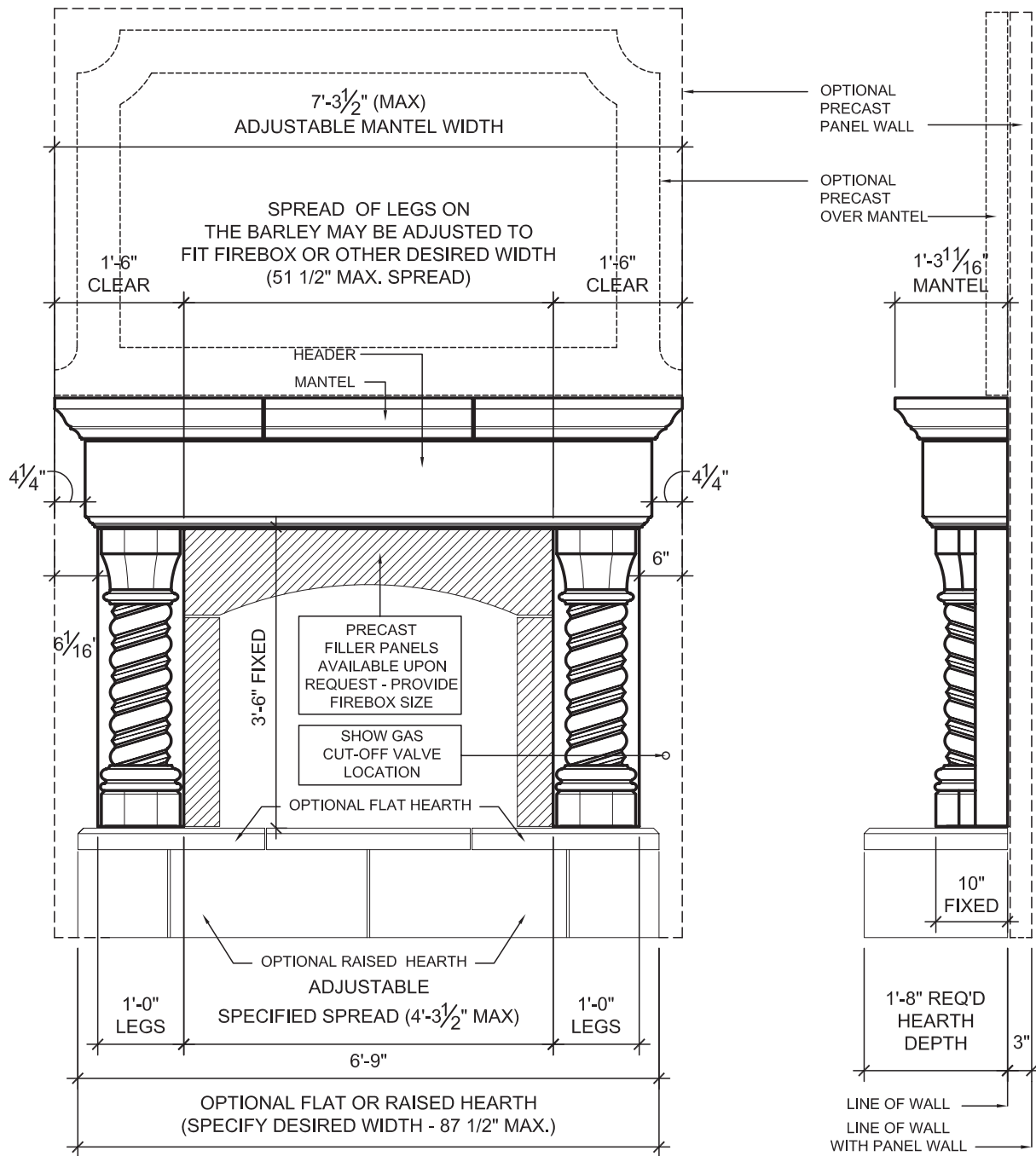
A ELEVATION - BARLEY FIREPLACE 1/2" = 1'-0"
