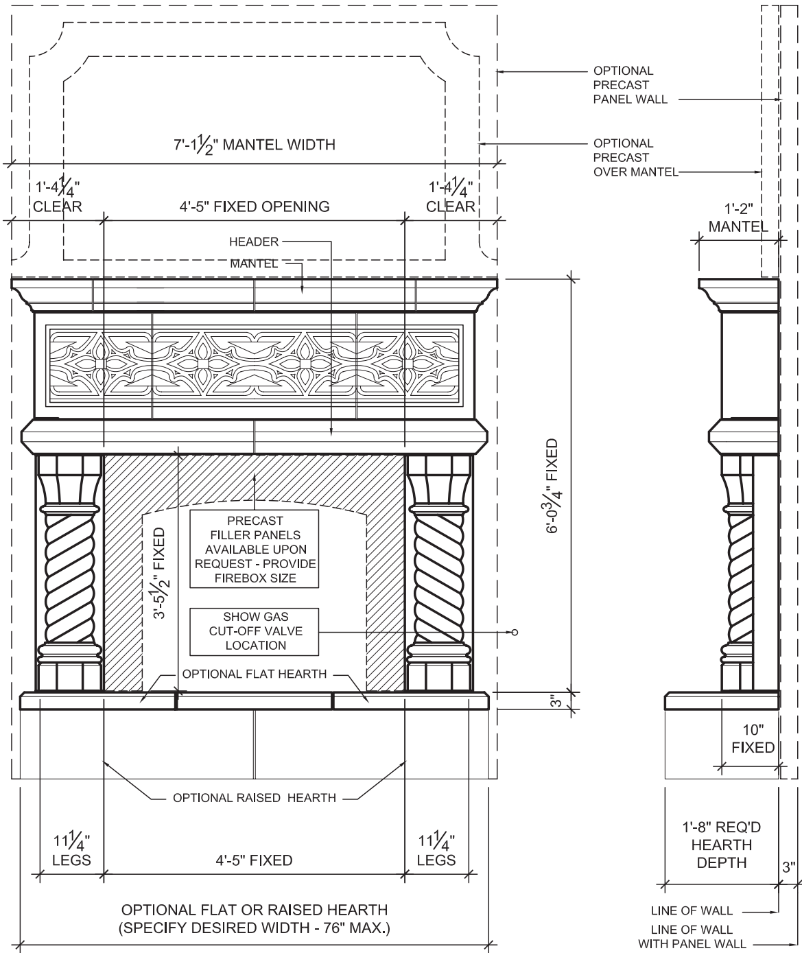
(B) SIDE 1/2" = 1'-0"
