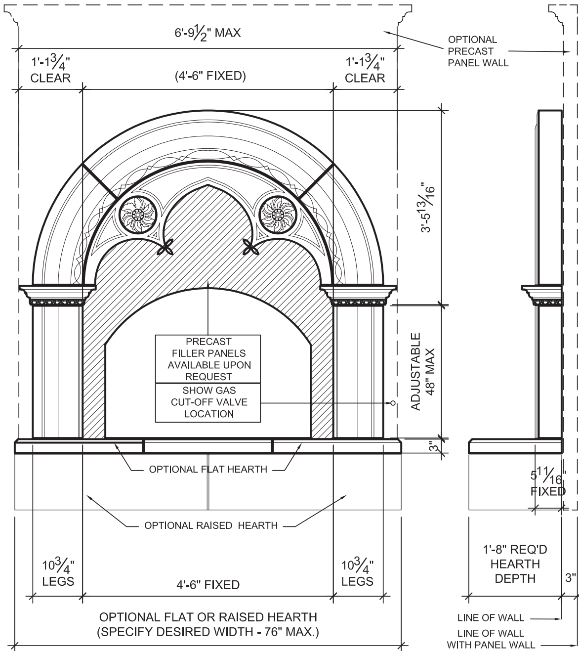
A ELEVATION BYZANTINE FIREPLACE 1/2" = 1'-0"
