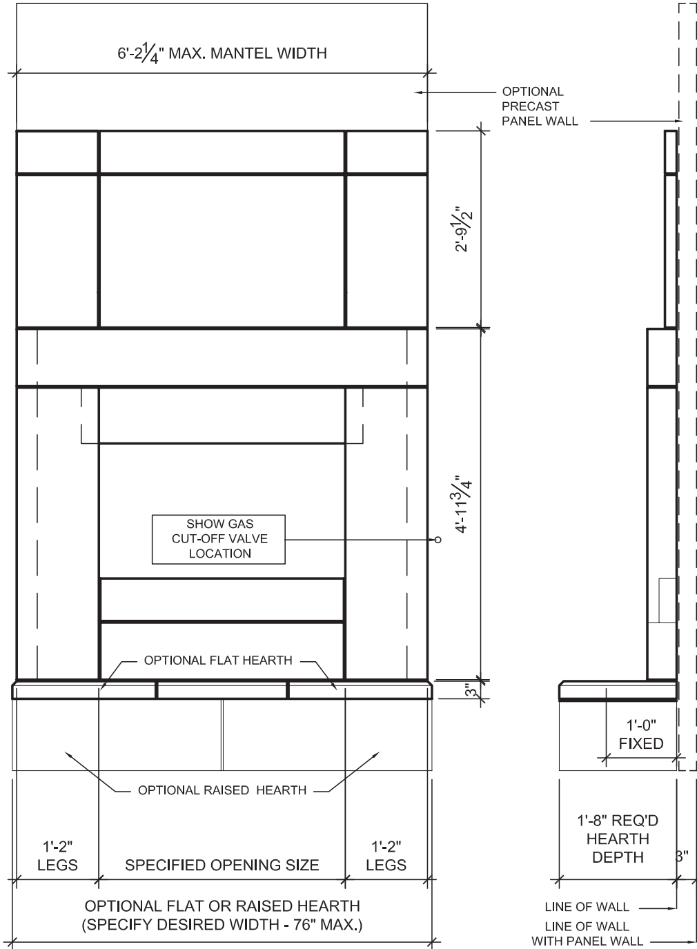
(A) ELEVATION - CONTEMPO FIREPLACE 1/2" = 1'-0"
