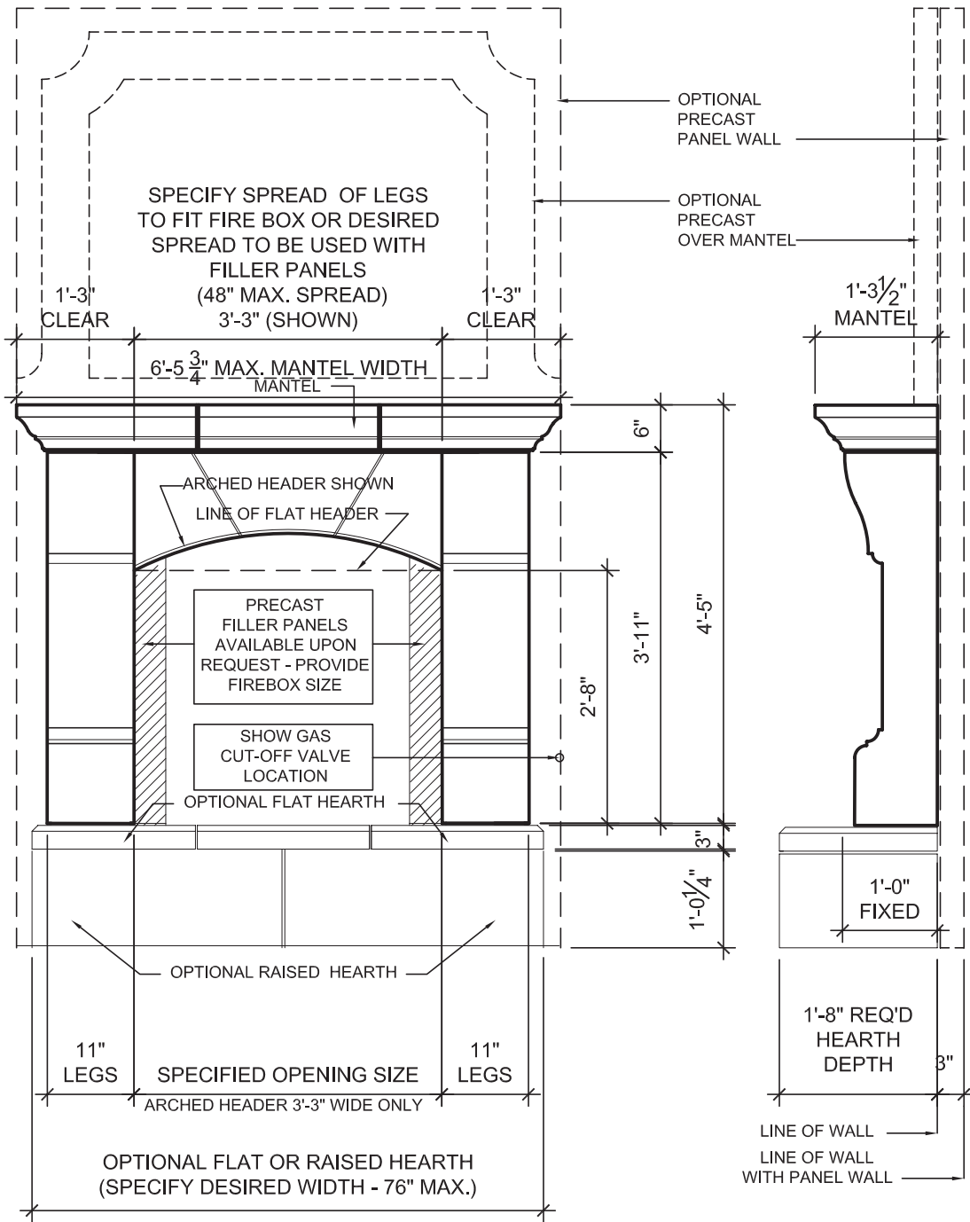
(A) ELEVATION - DEVONSHIRE 1/2" = 1'-0"
