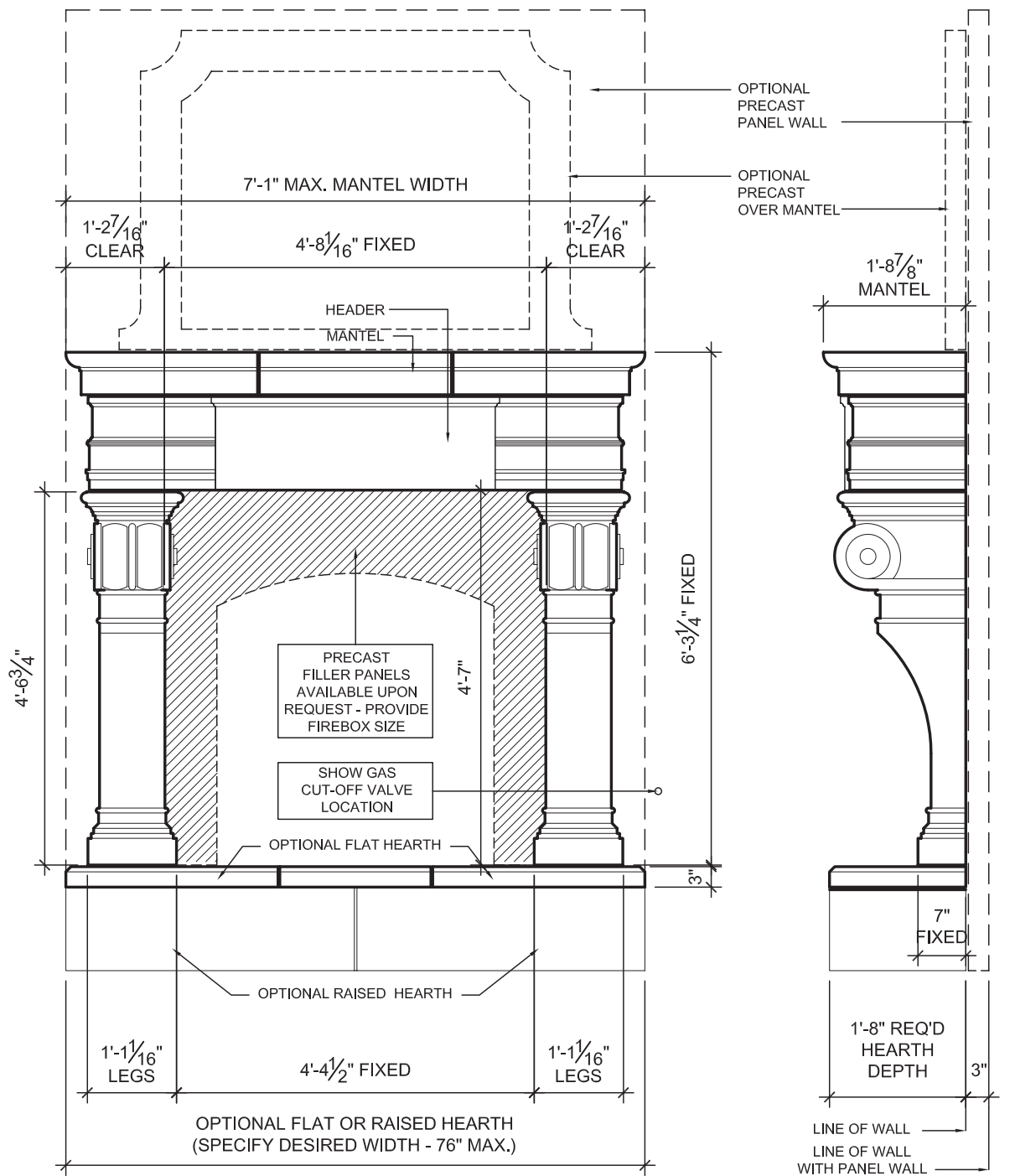
(A) ELEVATION - FLORENTINE FIREPLACE 1/2" = 1'-0"
