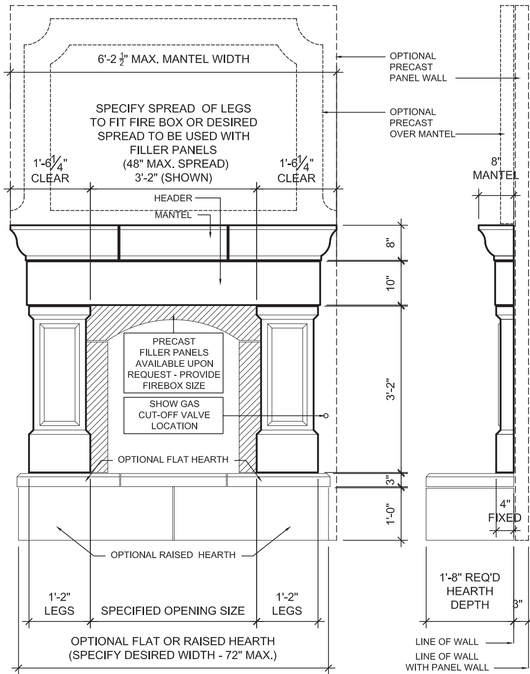
(A) ELEVATION - GRACELAND FIREPLACE 1/2" = 1'-0"
