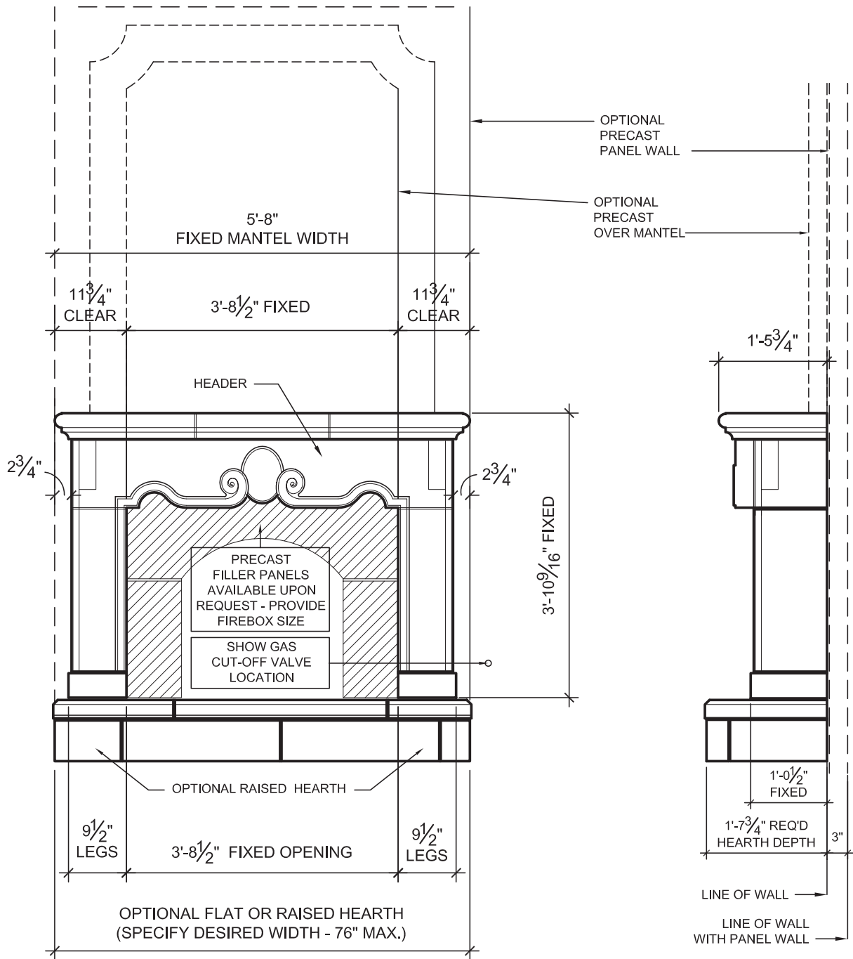
(A) ELEVATION - ISABELLA FIREPLACE 1/2" = 1'-0"
