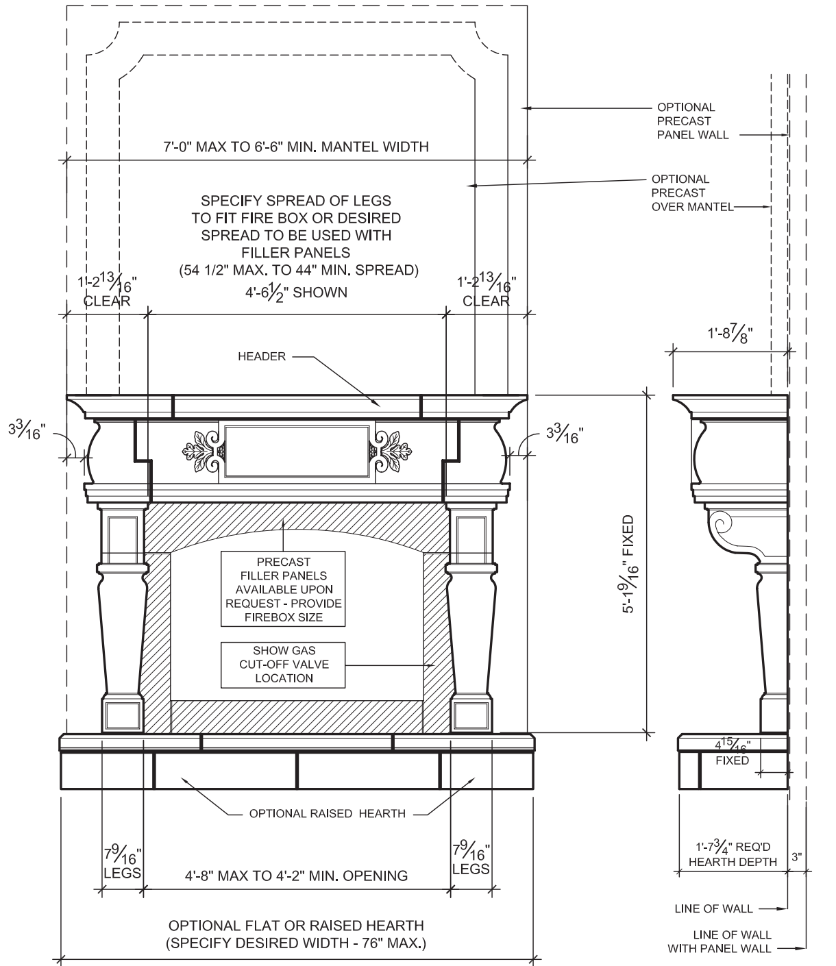
A ELEVATION - JARDIN FIREPLACE 1/2" = 1'-0"
