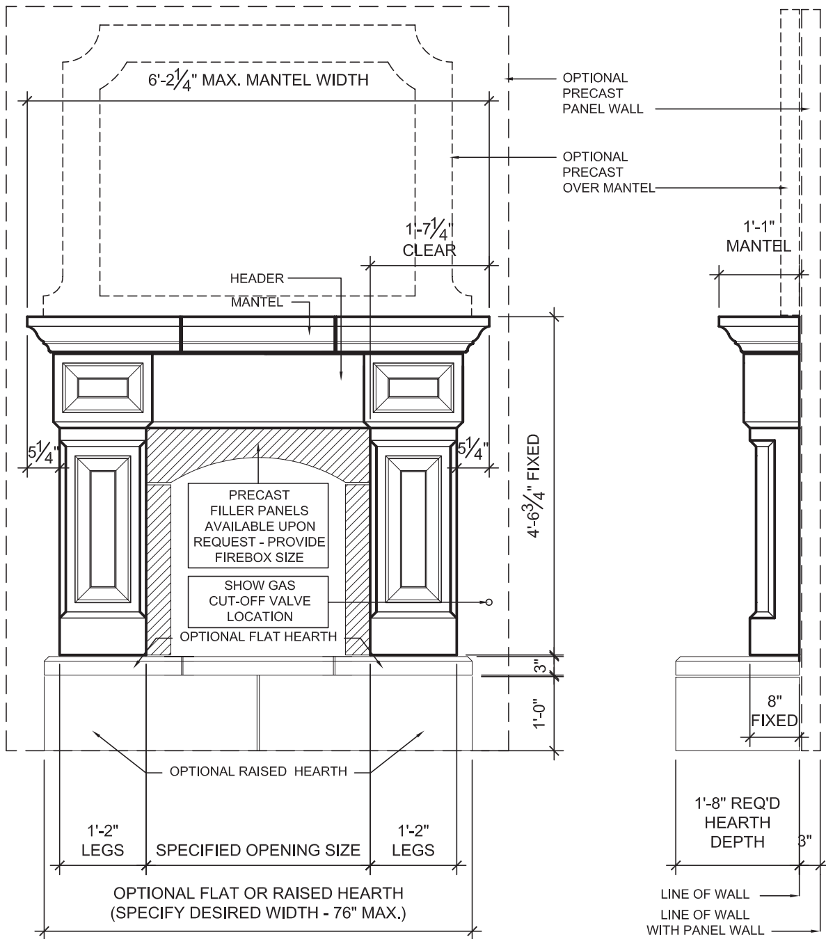
(B) SIDE 1/2" = 1'-0"
