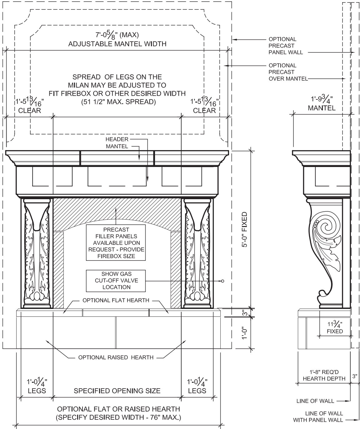
(A) ELEVATION - MILAN FIREPLACE 1/2" = 1'-0"
