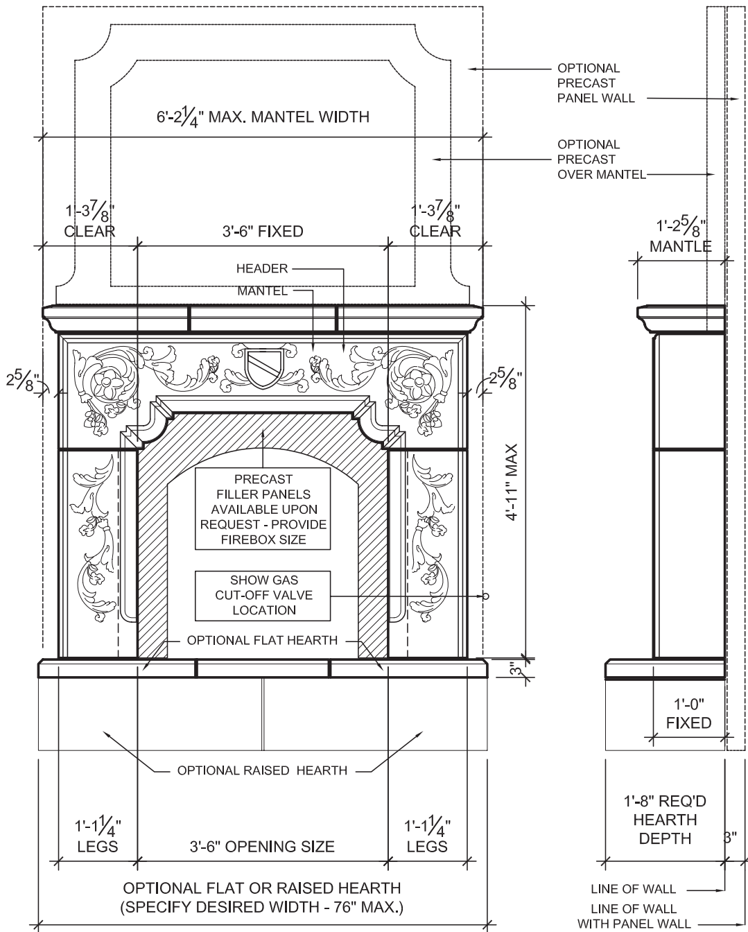
A ELEVATION - MONACO FIREPLACE 1/2" = 1'-0"
