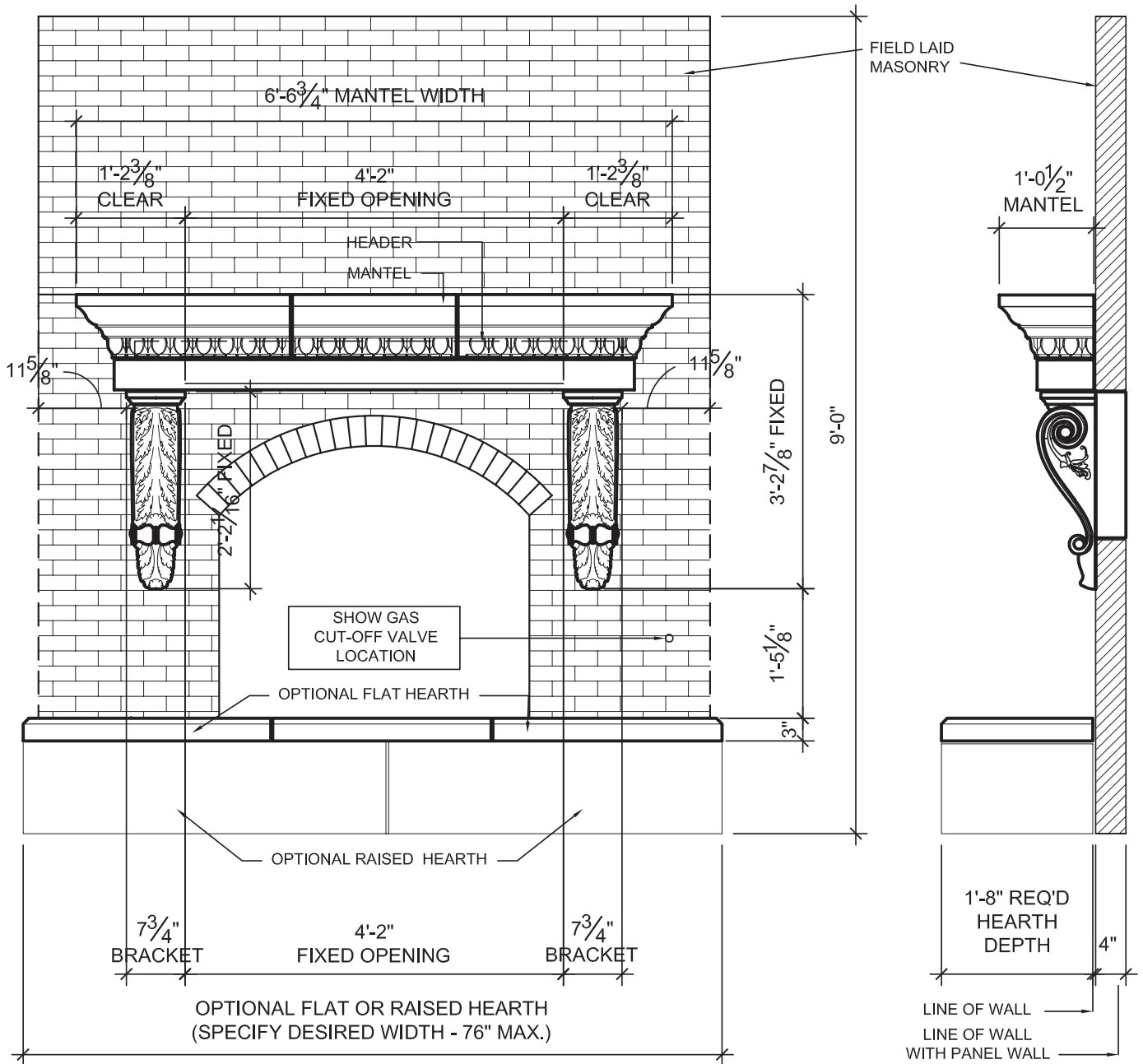
(B) SIDE 1/2" = 1'-0"
