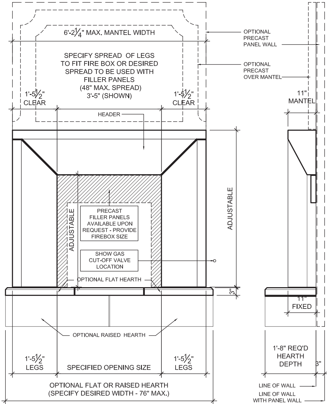
(A) ELEVATION - NEWPORT FIREPLACE 1/2" = 1'-0"
