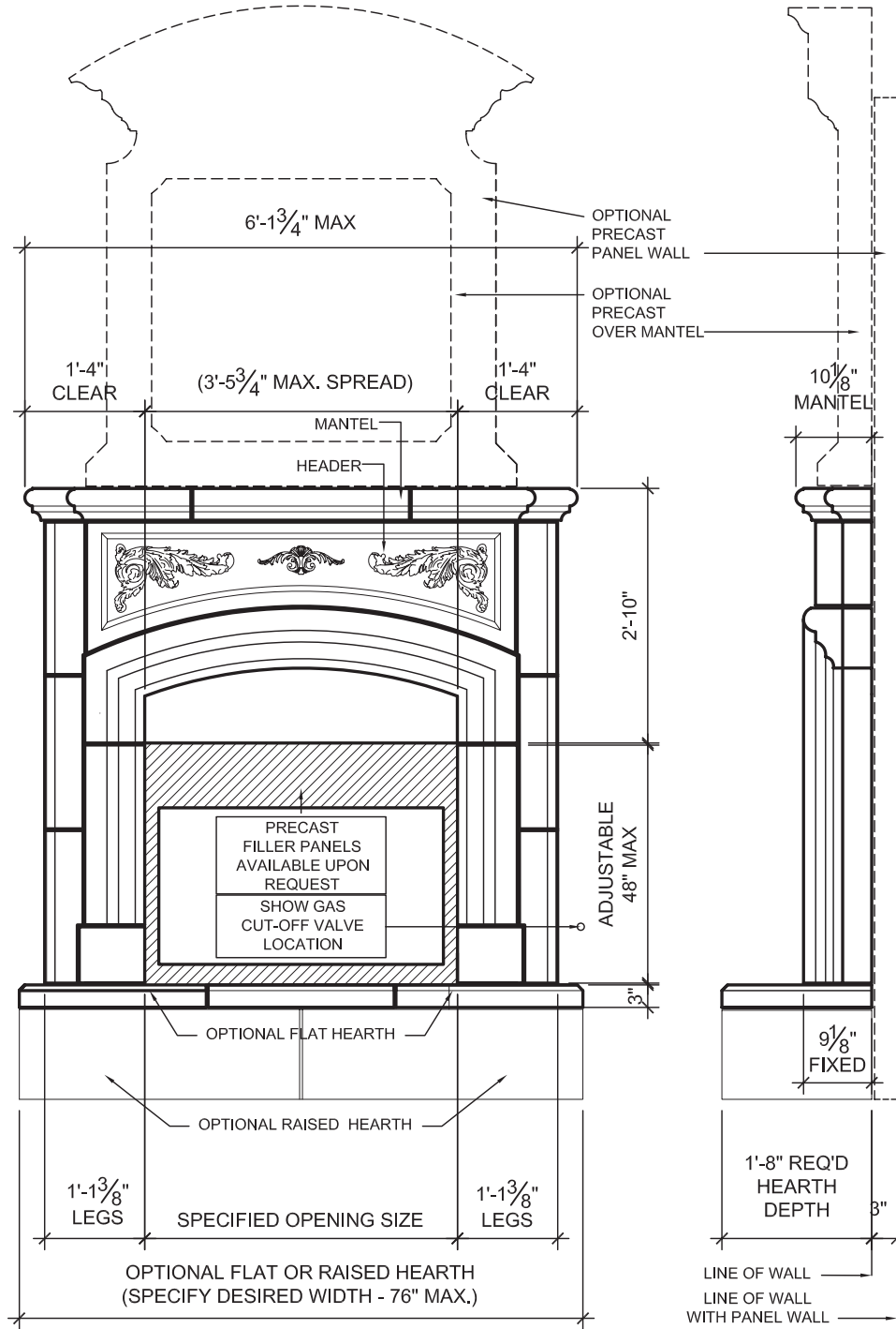
A ELEVATION - PORTABELLO FIREPLACE 1/2" = 1'-0"
