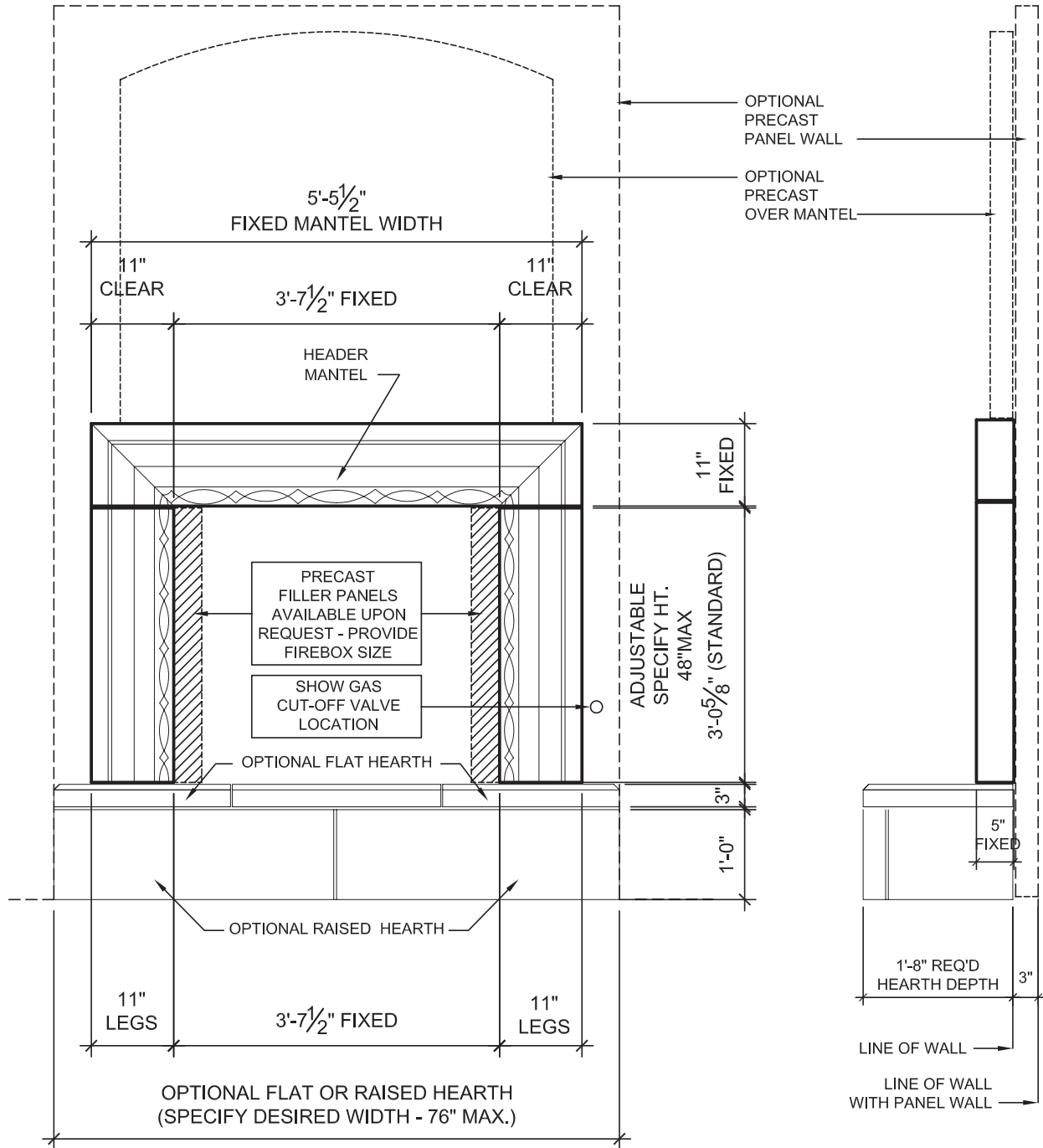
A ELEVATION - ROCOCO FIREPLACE 1/2" = 1'-0"
