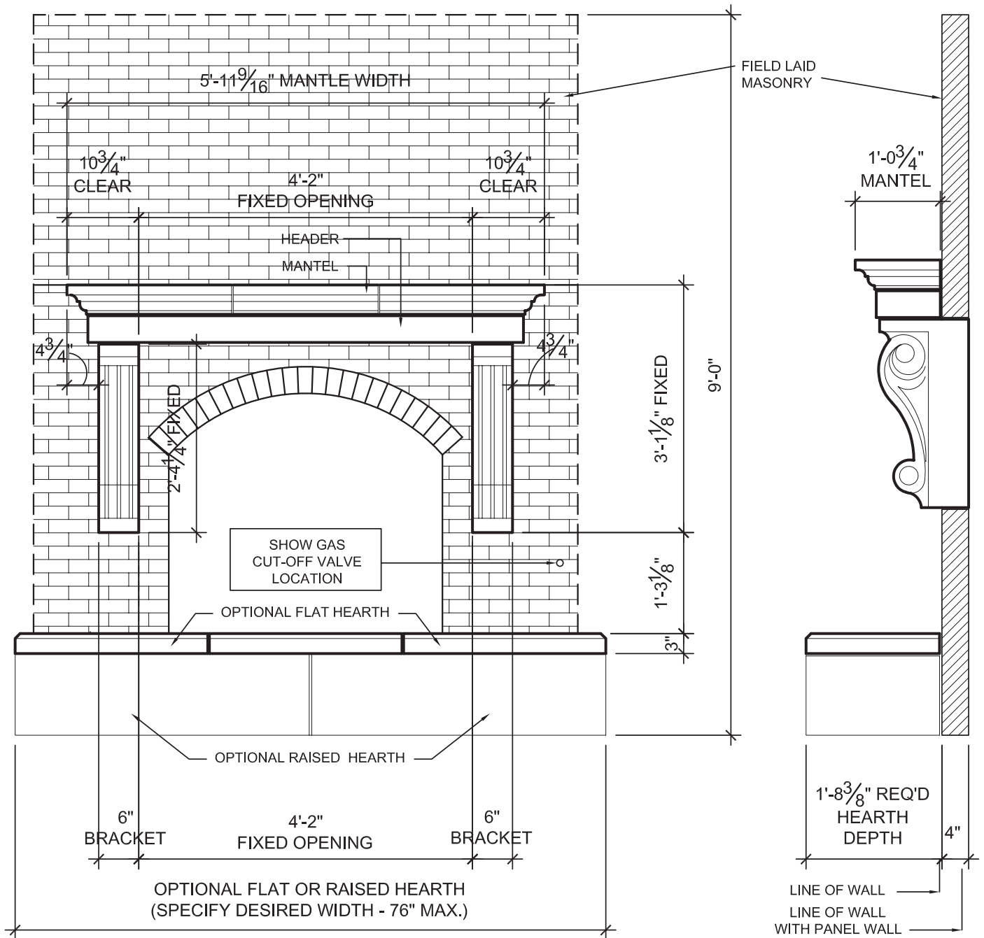
(B) SIDE 1/2" = 1'-0"
