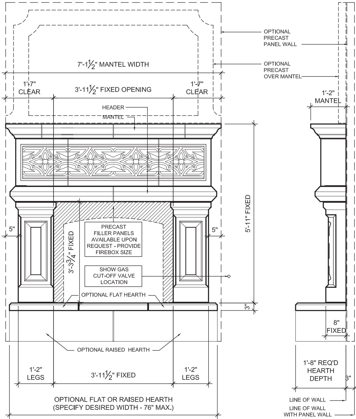
A ELEVATION - SAVOY FIREPLACE 1/2" = 1'-0"
