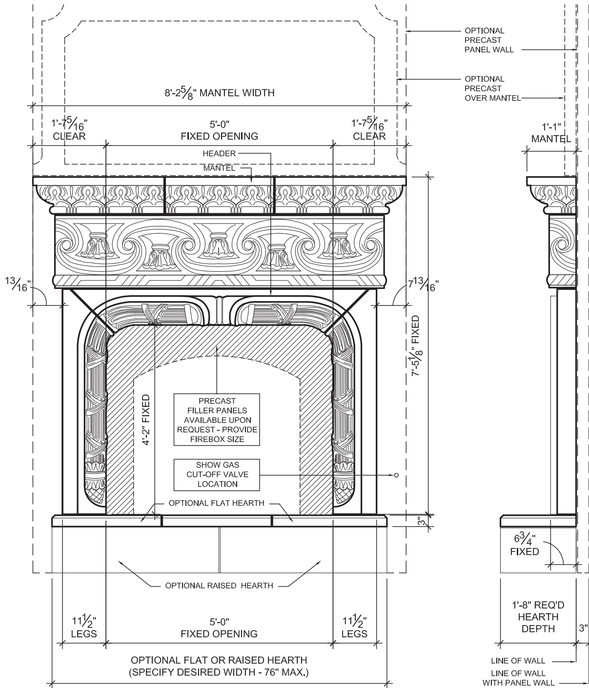
A ELEVATION - SOLOMAN FIREPLACE 1/2" = 1'-0"
