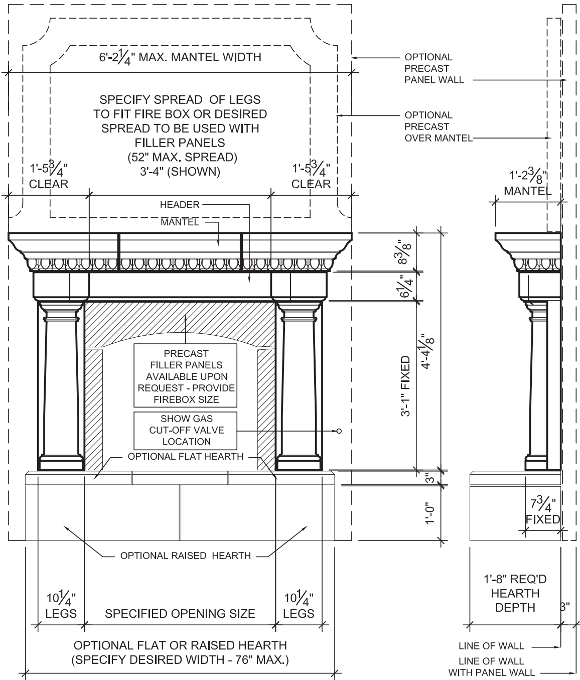
(A) ELEVATION - TUSCANY FIREPLACE 1/2" = 1'-0"
