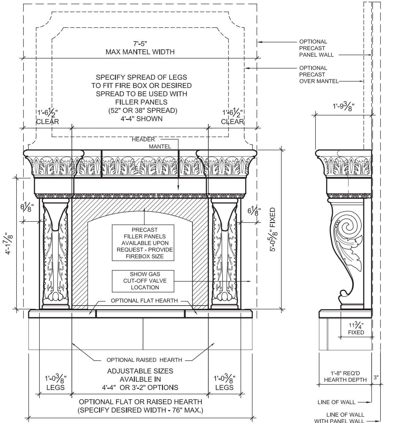
B SIDE 1/2" = 1'-0"
