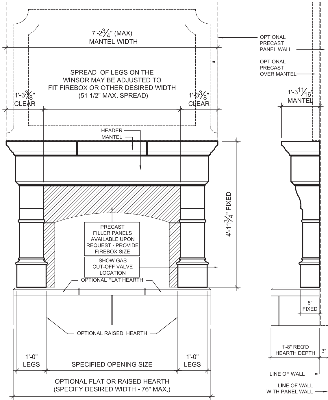
(A) ELEVATION - WINSOR FIREPLACE 1/2" = 1'-0"
