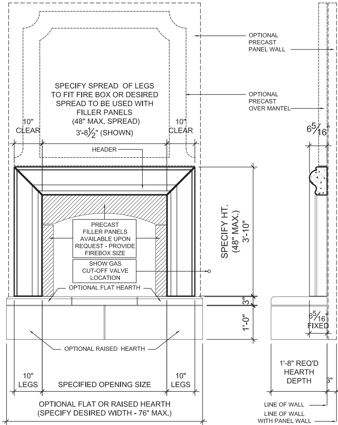
B SECTION 1/2" = 1'-0"
