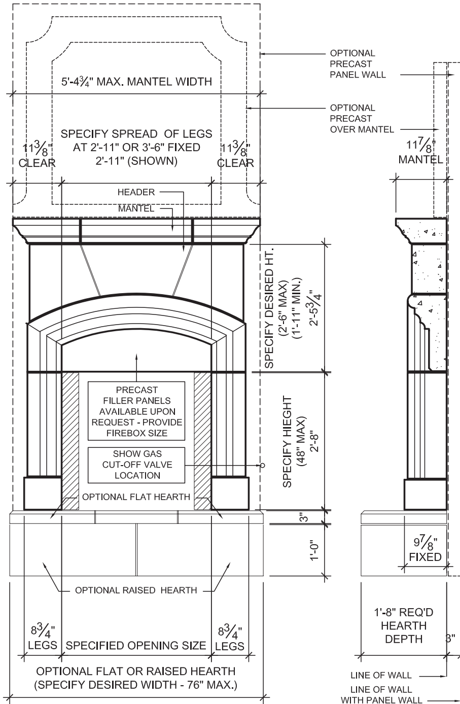
A ELEVATION - YORKSHIRE A FIREPLACE 1/2" = 1'-0"
