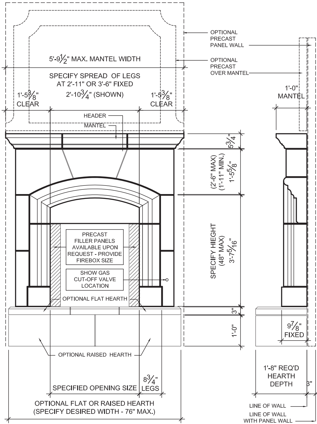
A ELEVATION - YORKSHIRE FIREPLACE 1/2" = 1'-0"
