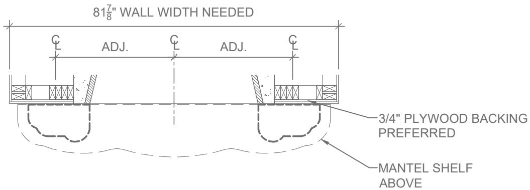
3 FRAMING PLAN SCALE: 1/2"=1'-0"
