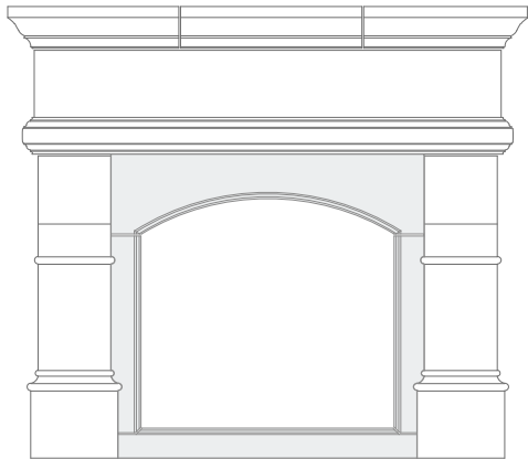
OGEE EDGE, EYEBROW FILLER PANEL **
